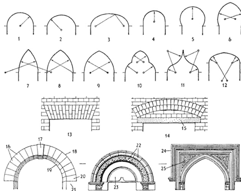
TYPES AND CONSTRUCTION OF ARCHES 1. Semicircular. 2. Segmental. 3. Elliptical. 4. Stilted. 5. Round horseshoe. 6. Pointed horseshoe. 7. Lancet. 8. Equilateral. 9. Drop. 10. Trefoil or cusped. 11. Ogee. 12. Four-centred. 13. Flat arch. 14. Relieving arch. 15. Lintel. 16. Voussoirs. 17. Keystone. 18. Extrados. 19. Intrados, soffit, or archivolt. 20. Springer. 21. Impost. 22. Orders. 23. Tympanum. 24. Hoodmould, dripstone, or label. 25. Spandrel
